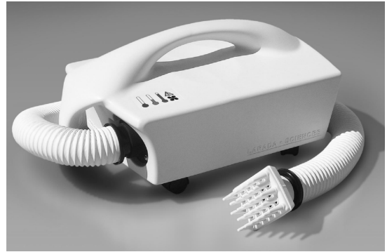
Fig. 2. The LouseBuster is a custom-built medical device designed to kill all life stages of head lice by delivering precisely controlled, heated air ( 59 \pm 1.5^\circ\text{C} ) at an airflow two to three times greater than that of a hand-held blow dryer. A removable hose directs the air through a disposable, diffuser-like applicator that distributes air to the scalp and bases of hair shafts, where lice and their eggs congregate. During treatment the applicator is held in overlapping positions on the scalp (30 s per position). A specific pattern is followed to ensure that all areas of the scalp receive adequate coverage. The entire scalp can be treated in \approx 30 min, independent of hair length.
